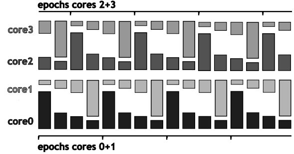
Figure 4. Sorted scheduling. Bars correspond to memory intensity.
